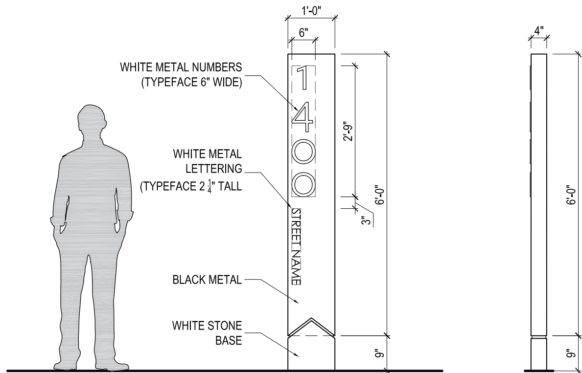
White / stainless steel pin-mounted letters with backlit illumination
